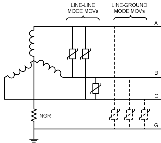
Fig. 2 TVSS for High Resistance Grounded System
