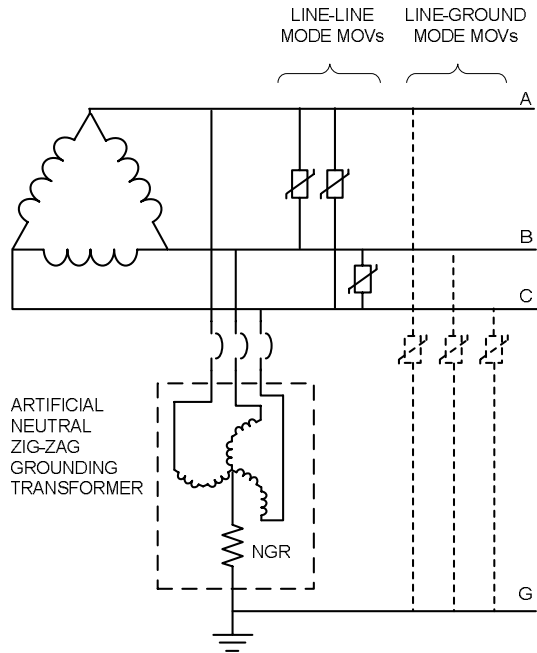
Fig. 3 High Resistance Grounding of a Delta System
