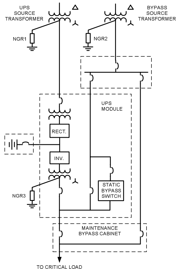
Fig. 5 Grounding of UPS Bypass Input and Inverter Output
