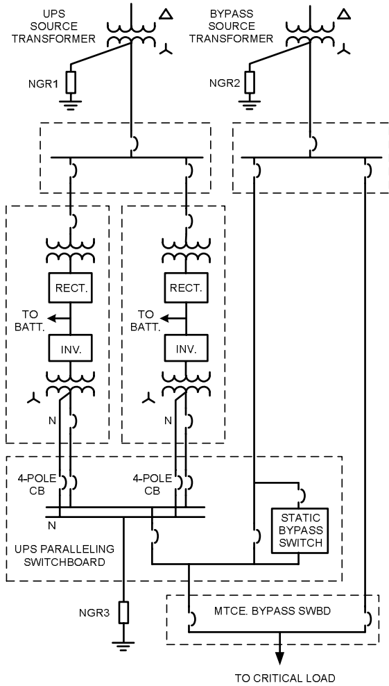
Fig. 6 High Resistance Grounding of a Parallel UPS System
