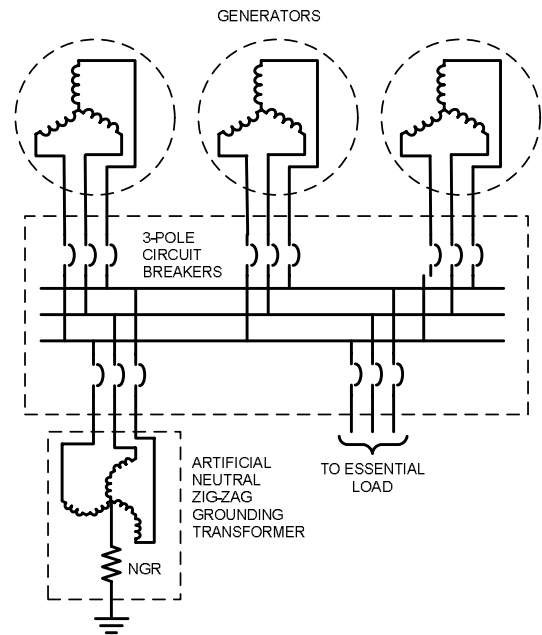
Fig. 7 High Resistance Grounding Scheme of Parallel Generators
