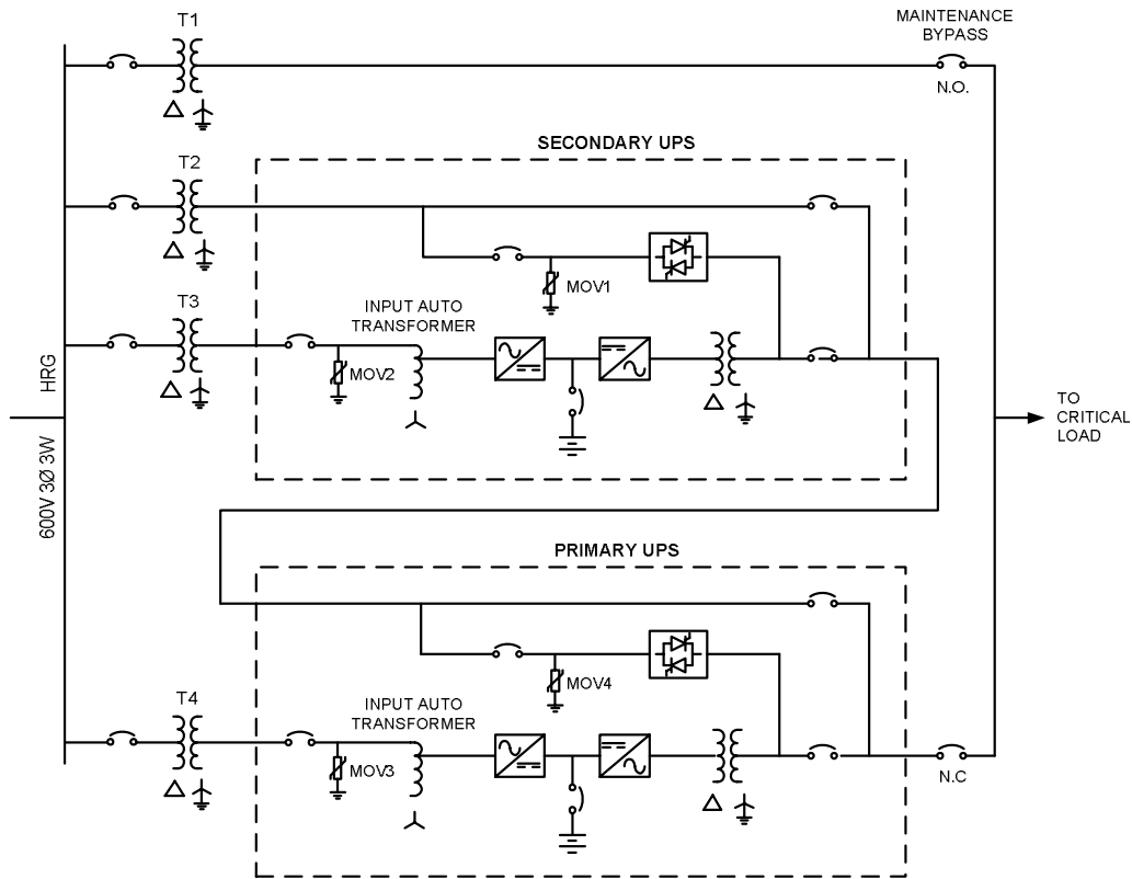
Fig. 4 Simplified One Line Diagram for Isolated Redundant UPS System.
